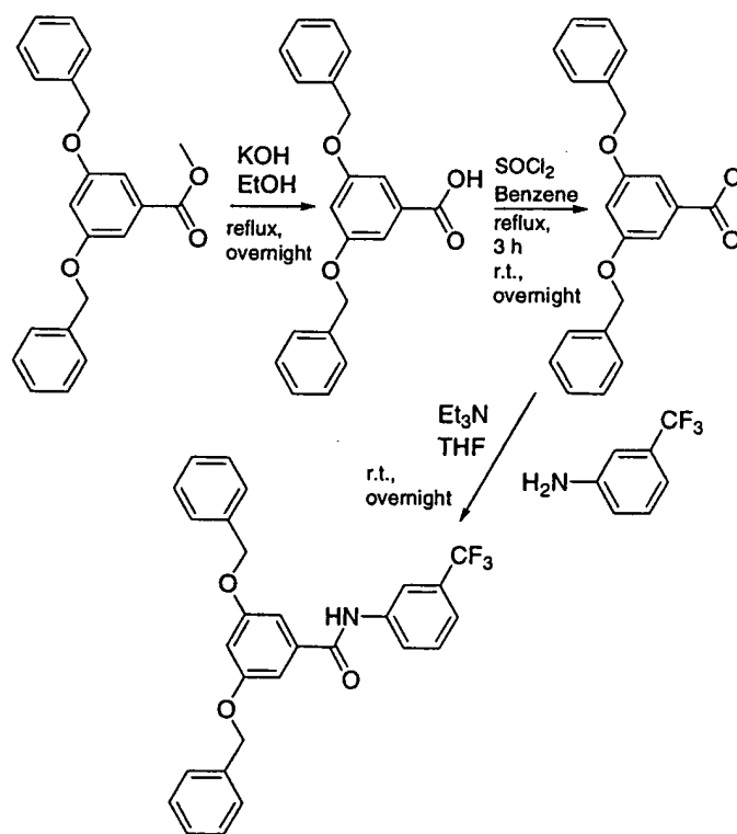
Scheme V
